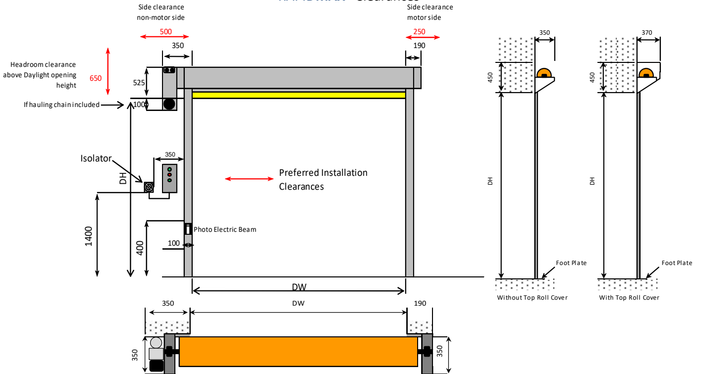
MAX Doors ISO-FLEX™ door curtain 240v Single Phase GfA SafeDrive®
